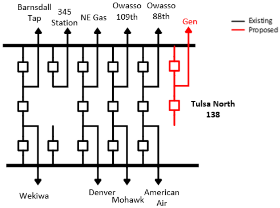
Figure 1: Point of Interconnection (POI INFORMATION) One-Line Diagram
